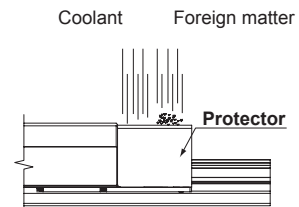
Configuration diagram of the inside the protector (Ex: in case of QZJJHH Type)
