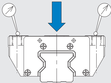
Radial rigidity
