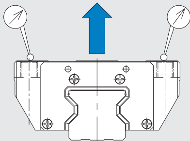
Reverse-radial rigidity
