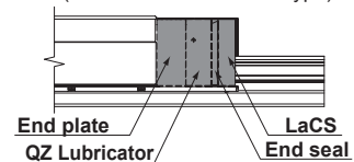
Configuration diagram of the inside the protector (Ex: in case of QZJJHH Type)
