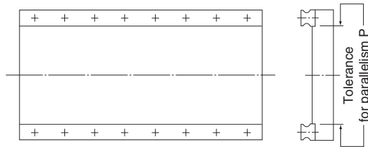
Error Allowance in Vertical Level (X) between Two Rails
