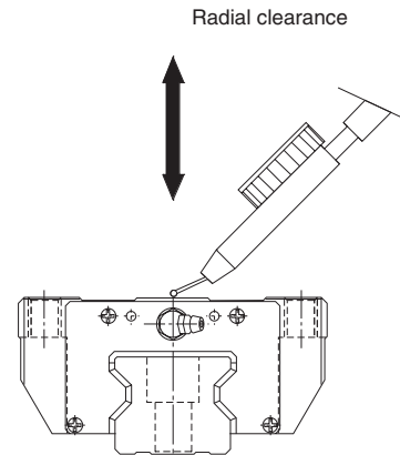
Radial clearance of models SRG/SRN
