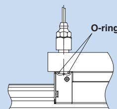
Method for using the greasing hole on the top face
