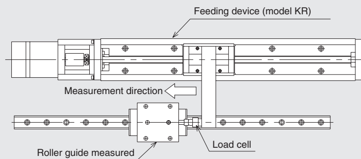
Rolling Resistance Measuring Equipment
